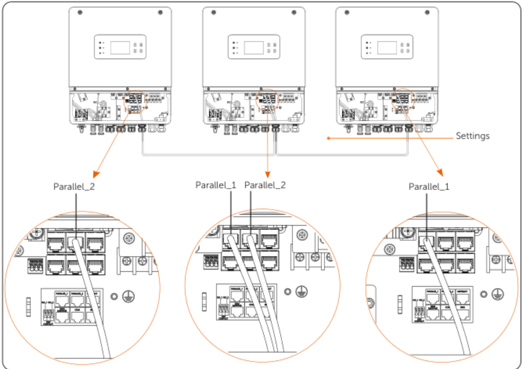
Parallel connection diagram
